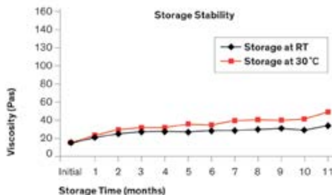
Figure 4 - Viscosity increase over time.
